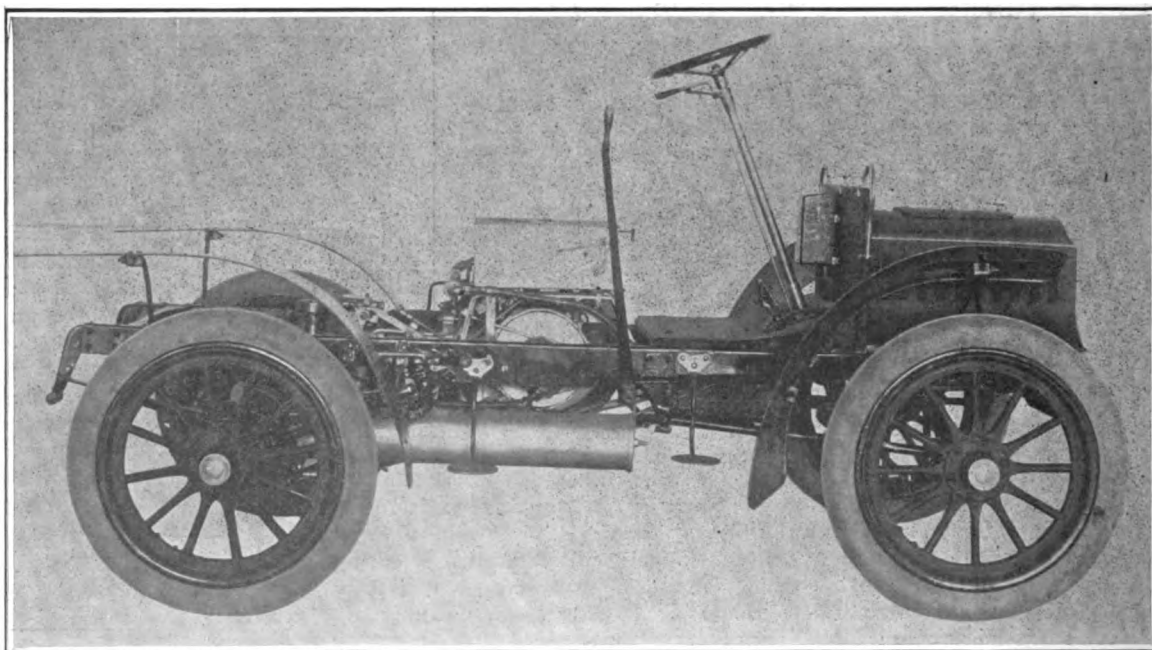
CADILLAC MODEL F CHASSIS, FOR SIDE-ENTRANCE TOURING BODY OR DELIVERY WAGON TOP.
